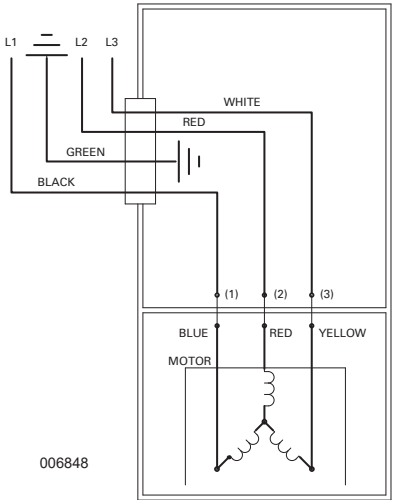
WIRING DIAGRAM FOR MODELS "J292", "F292", "G292" & "BA292" All Revisions
