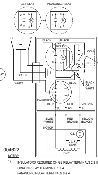
WIRING DIAGRAM FOR MODELS "D293-C" & "H293-C" 9/86 (VS) thru Current
