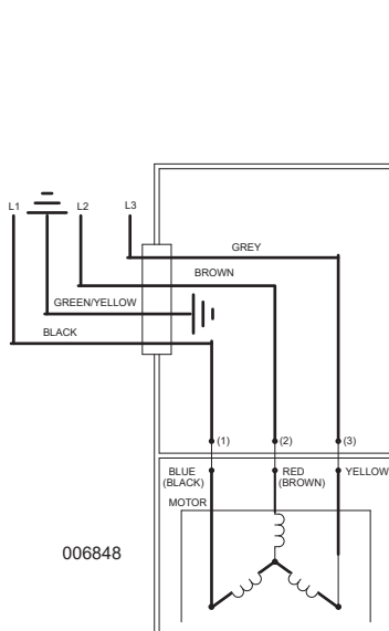
WIRING DIAGRAM FOR MODELS "F293", "G293", "J293" & "BA293" 9/96 thru Current All Revisions
