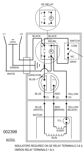
WIRING DIAGRAM FOR MODELS "D293-A", "D293-B", "H293-A" & "H293-B" 12/80 (YJ) thru 8/86 (US)
