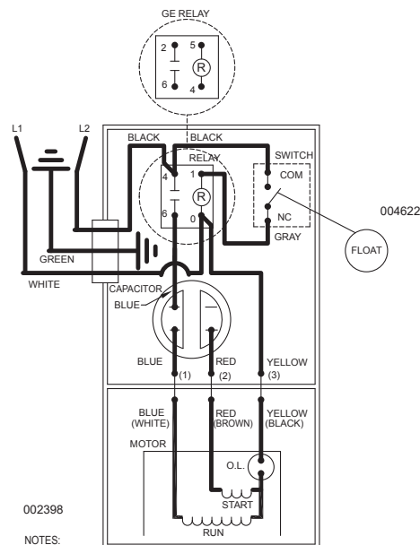
WIRING DIAGRAM FOR MODELS "M163-B" and "M163-C" "D163-A", "D163-B", "D163-C" 1/83 (MO) thru 8/86 (US)
