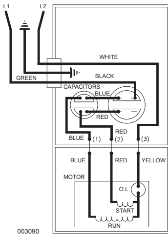
WIRING DIAGRAM FOR MODELS "N163-A" "E163-A" 4/81 (PM) thru 12/82 (YN)
