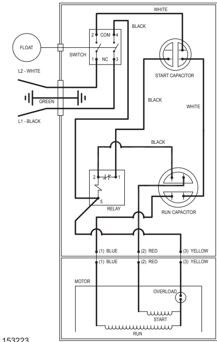
WIRING DIAGRAM FOR MODELS "M803", "M805", "M807", "D803", "D805", "D807" "DH803", "DH805", "DH807" 4/15 thru Current
