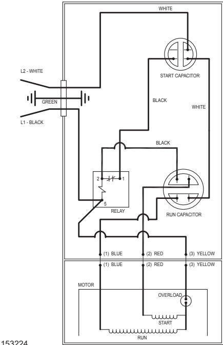
WIRING DIAGRAM FOR MODELS "N803", "N805", "N807", "E803", "E805", "E807" "EI803", "EI805", "EI807" 4/15 thru Current
