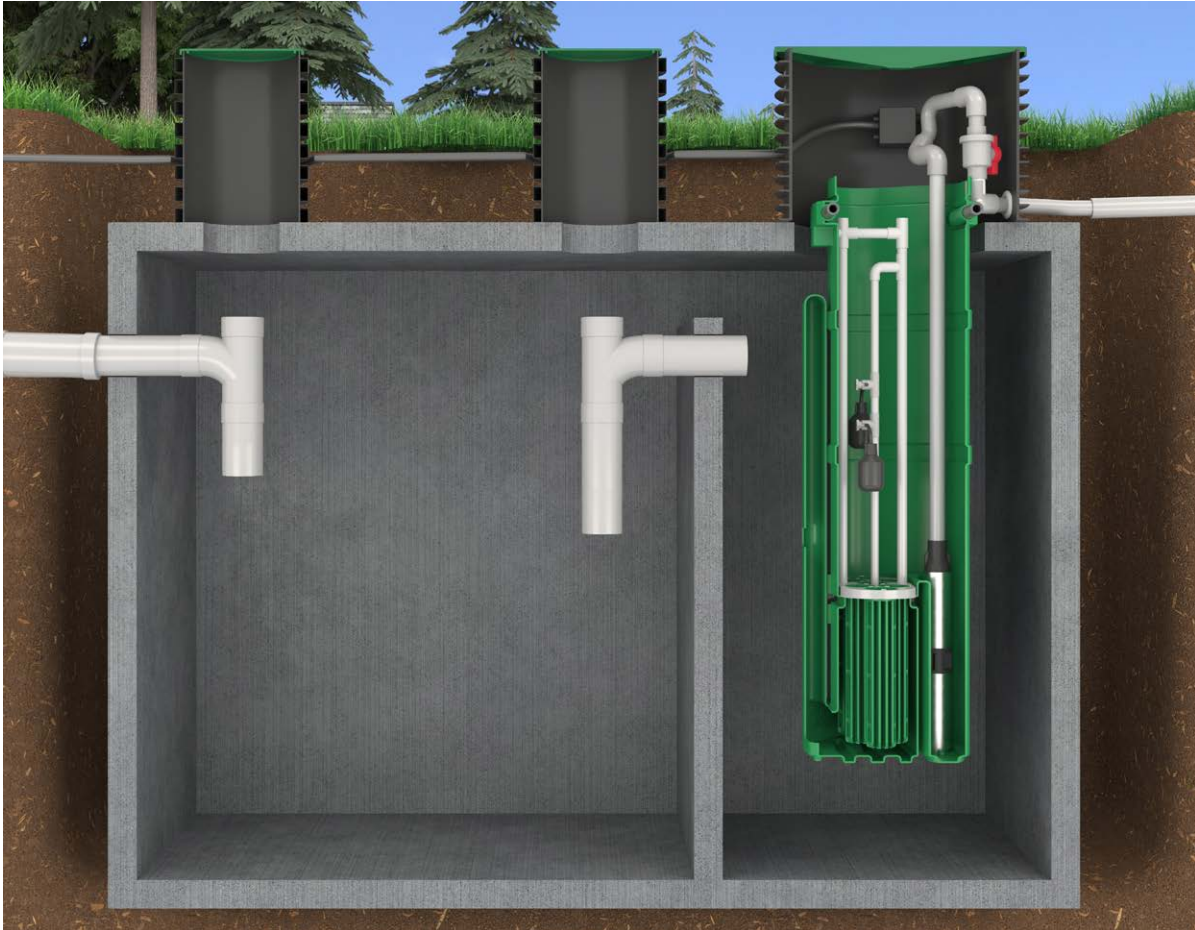
STEP (Septic Tank Effluent Pump) vaults are a common installation method for turbine pumps, featuring a built-in filter that's easily removed for cleaning.
