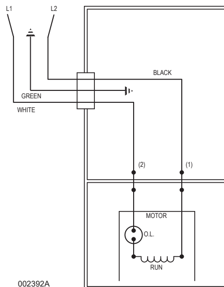
WIRING DIAGRAM FOR MODELS
