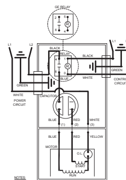
WIRING DIAGRAM FOR MODEL XE405 ALL REVISIONS
