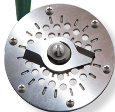
Grinder blade and cutting plate
