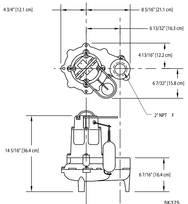
DIMENSIONAL DRAWING
