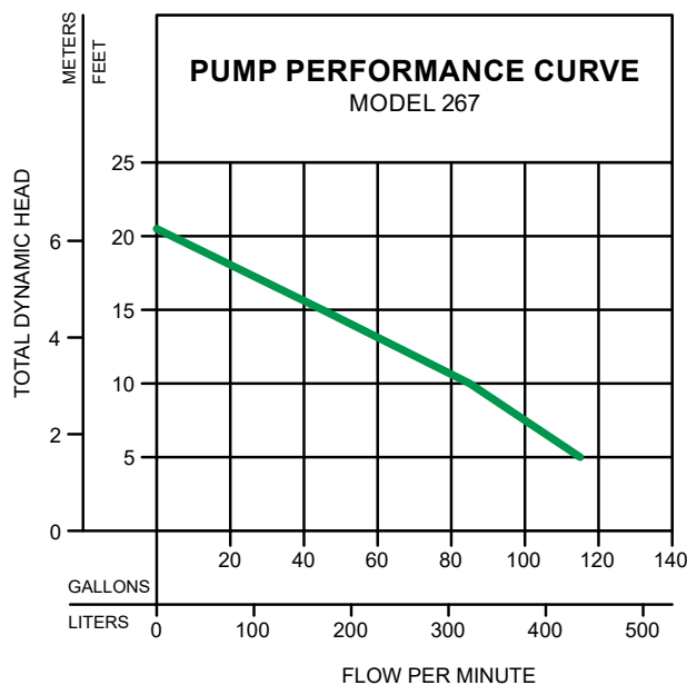
TOTAL DYNAMIC HEAD/FLOW PER MINUTE
