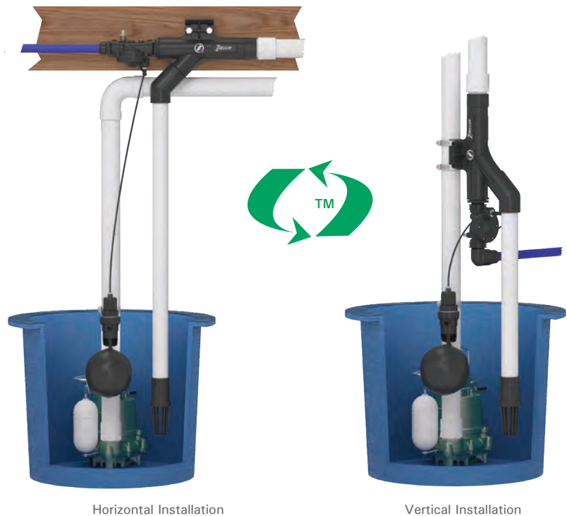
Horizontal Installation
